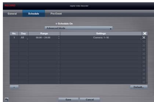
< Advanced Mode >
