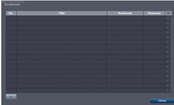
Figure 47: Bookmarks screen.
