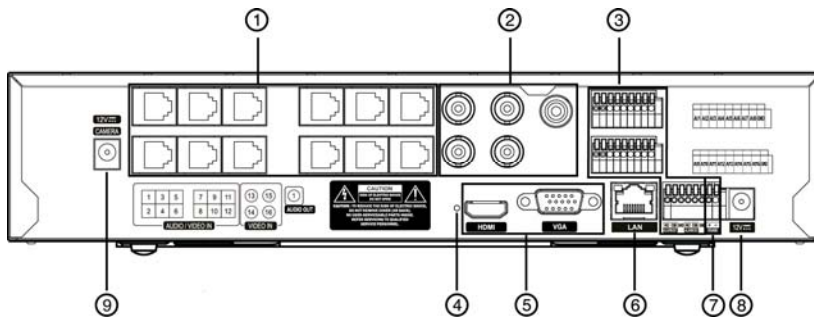
Figure 2: DVR rear panel.
